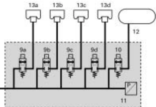
Magnetventilblock
